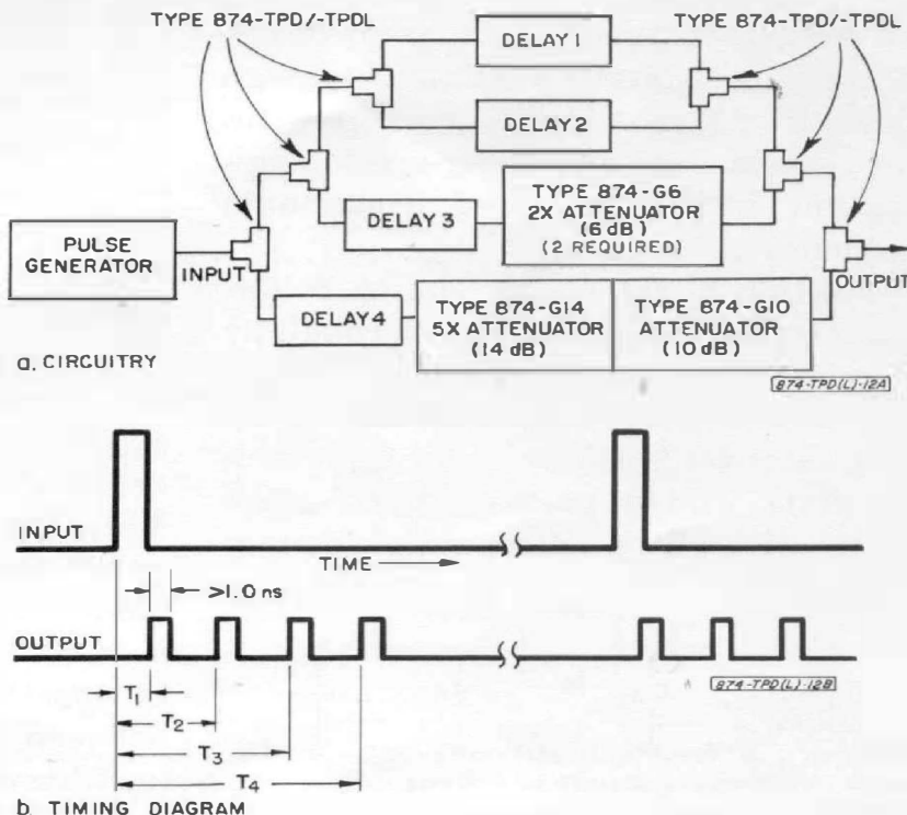
Figure 10. Cascaded power dividers used to construct a pulse burst, which effectively raises the repetition rate of a subnanosecond-rise-time pulse generator to several hundred megahertz.
