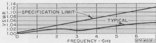
Figure 6. Type 874-W50B Termination VSWR.
