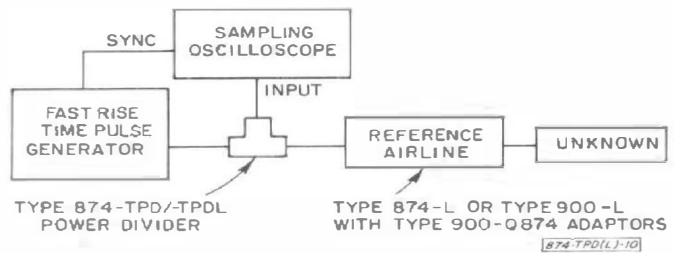
Figure 8. Use of the Type 874-TPDL/-TPD Power Divider in time-domain reflectometry instrumentation built around a sampling oscilloscope.
