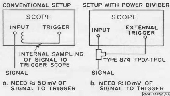
Figure 9. Use of the Type 874-TPDL/-TPD Power Divider to increase the sensitivity of sampling oscilloscopes.
