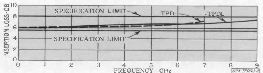
Figure 4. Typical insertion loss between center and side ports.
