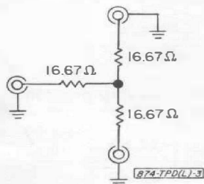
Figure 1. Simplified schematic of Power Divider.
