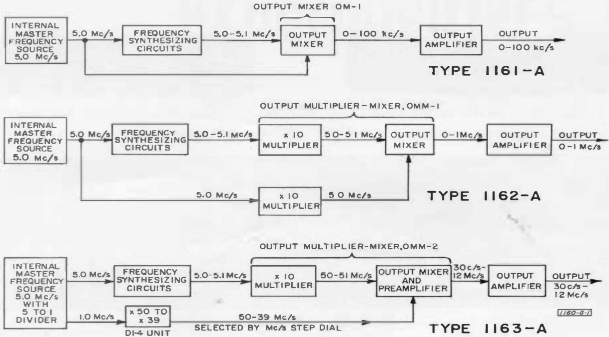
Figure 2. Block diagrams of the three GR synthesizers. All operate on the same principles and use interchangeable modules.
