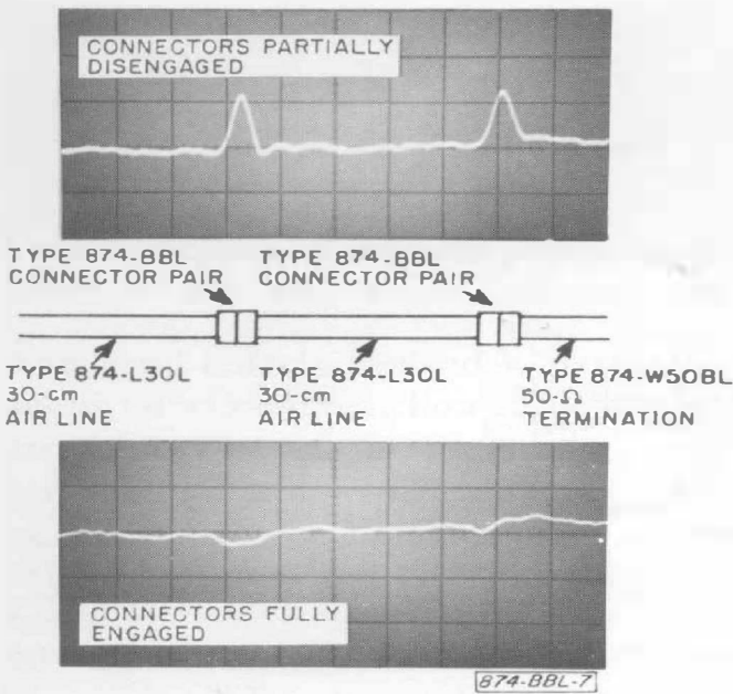
Figure 7. Time-domain reflectometer traces. Vertical scale: Reflection coefficient = 0.005/cm. ( Z_0 , normalized to 50 ohms, 1%/cm.) Horizontal scale: 6 cm of line/cm.
