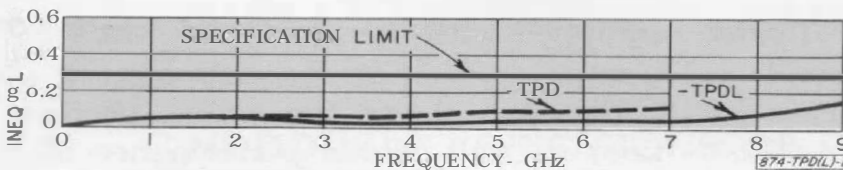
Figure 3. Typical inequality of output signals at side ports.
